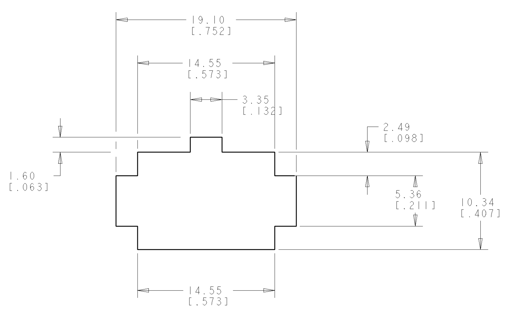
RECOMMENDED PANEL CUT OUT SCALE 4:1
