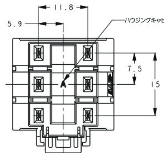
Receptacle Assembly
