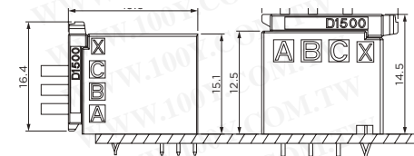
Horizontal/Vertical type
