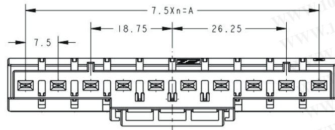
Receptacle Assembly
