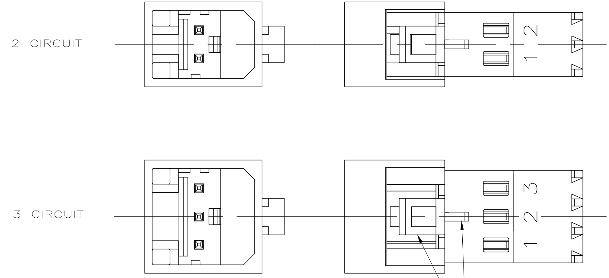
DETAIL A
