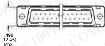
View of Rear Shell (With Shields Removed)
