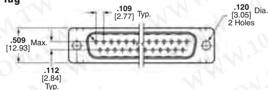
Plug
