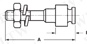
Part No. 747242-1
