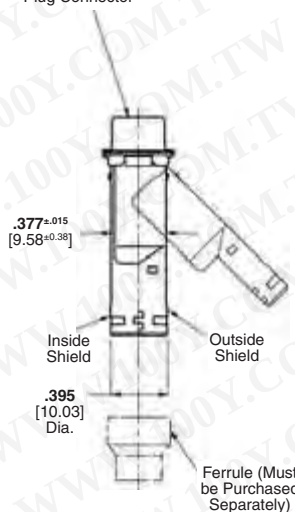
Plug Connector
