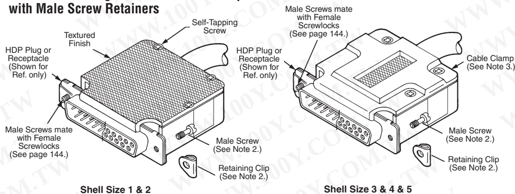
Shell Size 1 & 2
