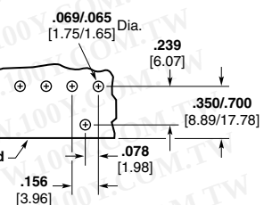
Recommended Mounting Hole Pattern for .062 [1.57] Thick PC Board Using a Right-Angle Header
