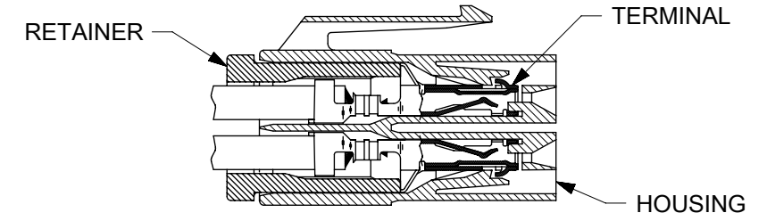
TERMINAL AND RETAINER ASSEMBLY DRAWING
