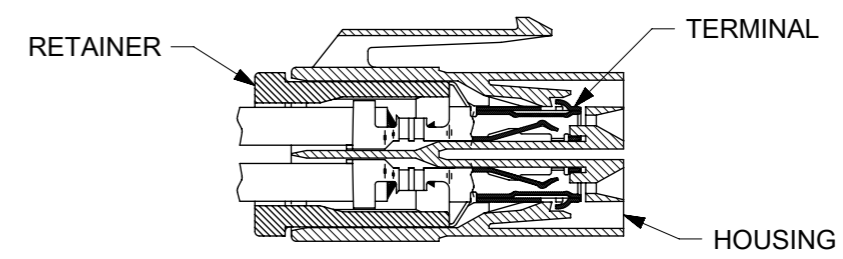
TERMINAL AND RETAINER ASSEMBLY DRAWING
