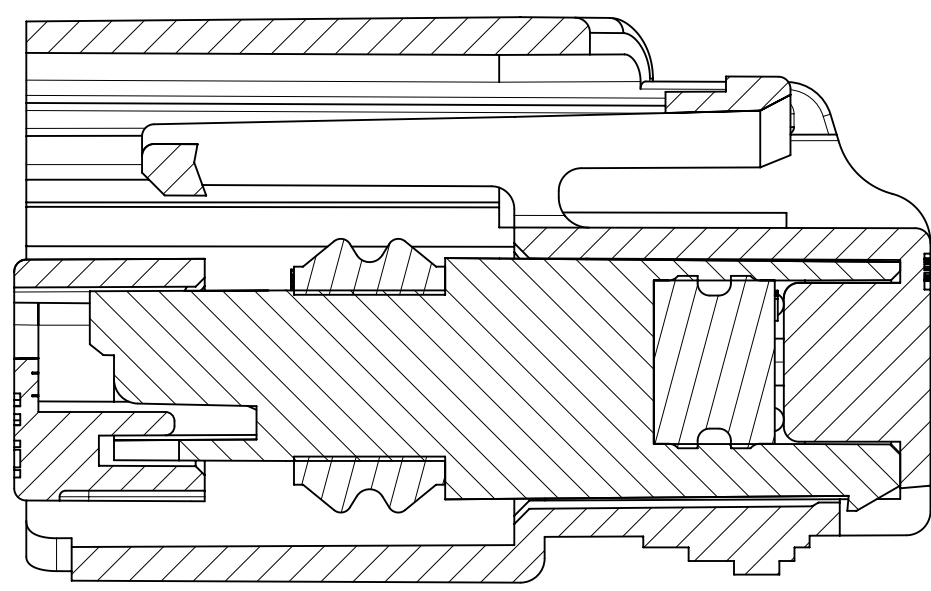
SECTION A-A TPA SHOWN IN AS-SHIPPED PRE-LOCKED POSITION SEE NOTE 1d
