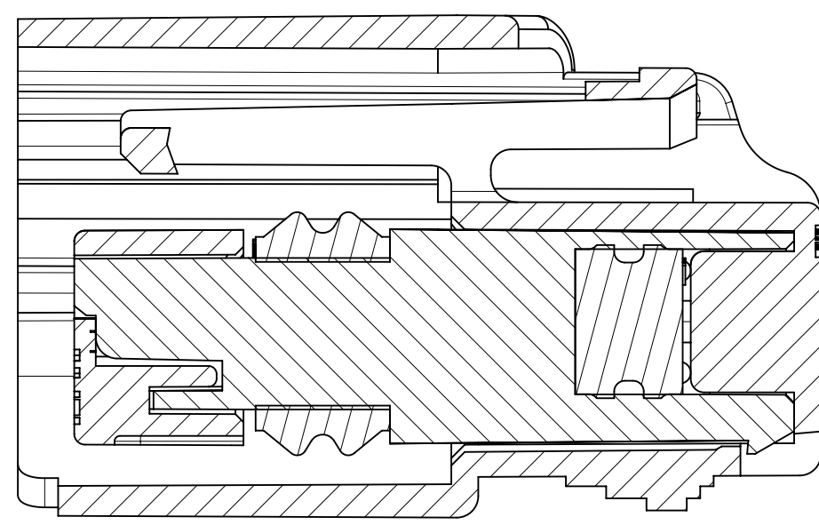
SECTION B-B TPA SHOWN IN FINAL LOCKED POSITION
