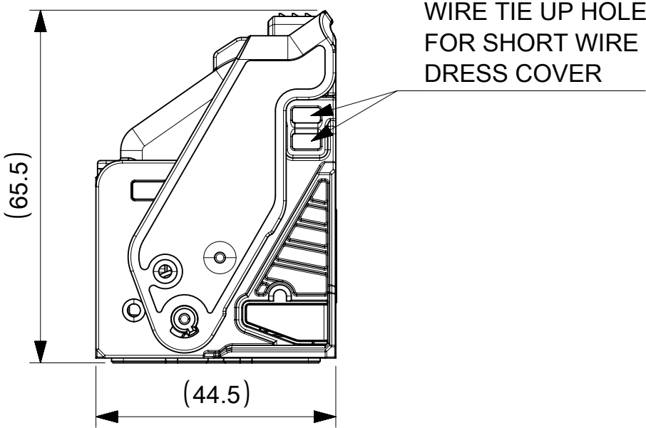
SHORT WIRE DRESS COVER
