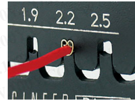
Precise crimping and excellent curling for conductor(wires) or sheath(insulator)
