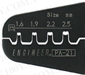
4-different cavities of elaborate dies
