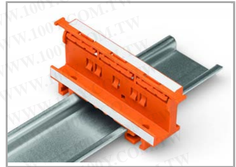
Mounting carrier on a DIN-35 rail
