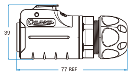
夹爪紧固式插头PE (外型尺寸图) PE clamping cable plug ( dimensions figure )
