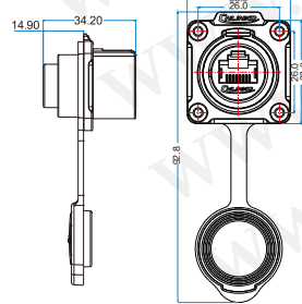
插座 SX (外型尺寸图) S socket ( dimensions figure )
