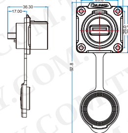
插座 SX (外型尺寸图) S socket ( dimensions figure )
