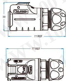
夹爪紧固式插头PE (外型尺寸图) PE clamping cable plug ( dimensions figure )
