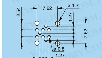
P19 - EPG-EXG (0B.309) Screw mount
