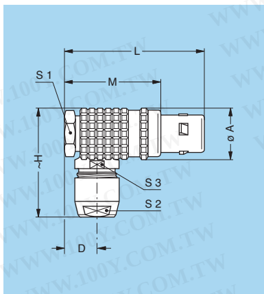
FHG Elbow (90°) plug, key (G) or keys (A...M and R), cable collet
