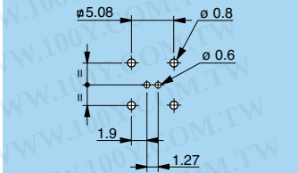
P19 - EPG-EXG (0B/1B.302) Screw mount
