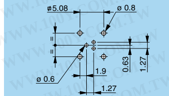
P19 - EPG-EXG (0B/1B.303) Solder mount
