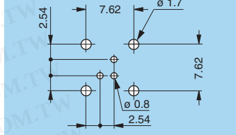
P19 - EPG-EXG (0B/1B.305) Screw mount
