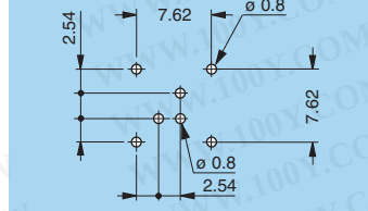
P19 - EPG-EXG (0B/1B.305) Solder mount
