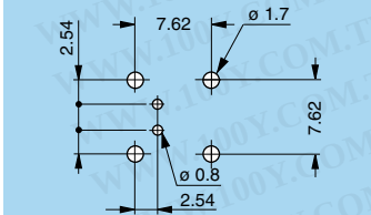
P19 - EPG-EXG (0B/1B.304) Screw mount
