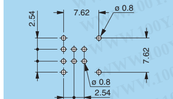
P19 - EPG-EXG (0B/1B.306) Solder mount
