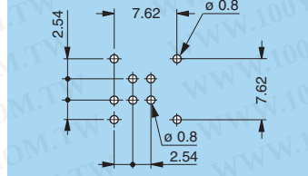
P19 - EPG-EXG (0B/1B.307) Solder mount
