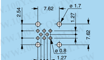
P19 - EPG-EXG (1B.308) Screw mount
