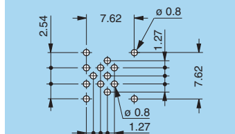
P19 - EPG-EXG (1B.310) Solder mount
