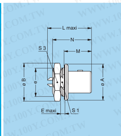
FAG Fixed plug, nut fixing, non-latching, key (G) or keys (A to F, L and R)
