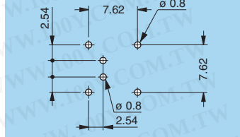
P19 - EPG-EXG (0B/1B.304) Solder mount
