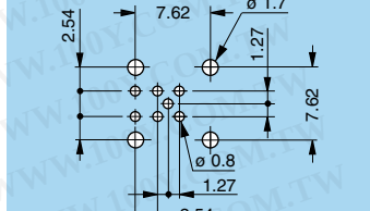
P19 - EPG-EXG (0B/1B.307) Screw mount
