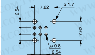
P19 - EPG-EXG (0B/1B.306) Screw mount
