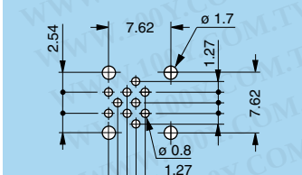
P19 - EPG-EXG (1B.310) Screw mount
