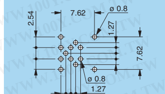
P19 - EPG-EXG (0B.309) Solder mount
