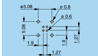
P19 - EPG-EXG (0B/1B.303) Screw mount
