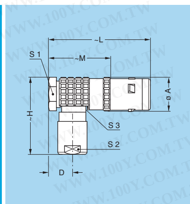
FPG Elbow (90°) plug, key (G) or keys (A to F, L and R), cable collet
