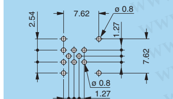
P19 - EPG-EXG (1B.308) Solder mount
