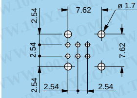
P22 - EPL - EXP Screw mount
