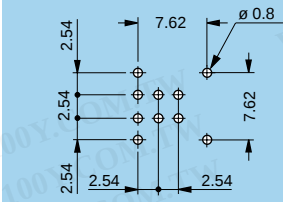
P22 - EPL - EXP Solder mount
