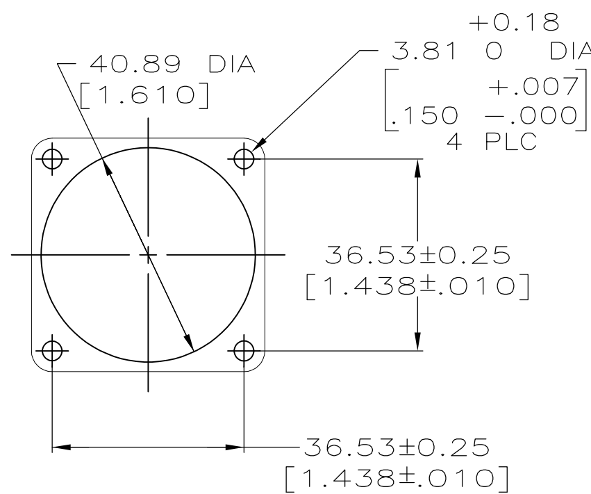
PANEL CUTOUT
