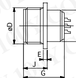
Flange Mount Receptacle
