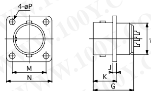
Flange Mount Receptacle
