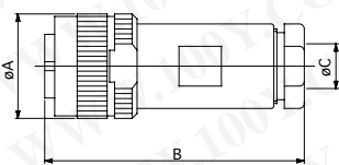
Plug / Normal Clamp Type
