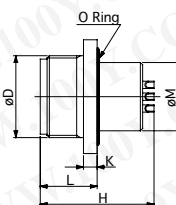
Flange Mount Receptacle
