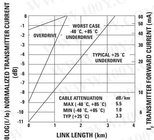
Figure 4. HFBR-14x2Z/HFBR-24x2Z Link Design Limits with 100/140 μm Cable.
