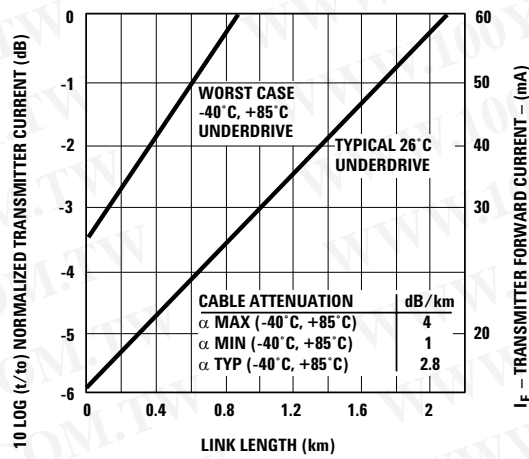
Figure 3. HFBR-1414Z/HFBR-2412Z Link Design Limits with 62.5/125 μm Cable.
