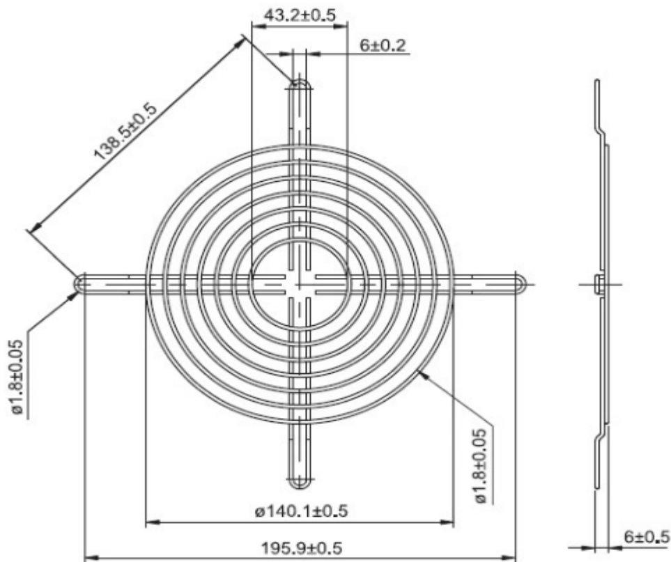
MG-16 (For UF16FC Series) *Steel
