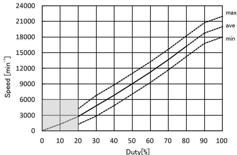
Referenc PWM Duty vs Speed Conditions : at rating Voltage, Vst=5.0V, f=25kHz, Ta=25°C
