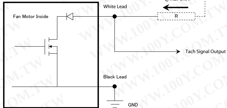
Fig. 1 Tach Signal Circuit
