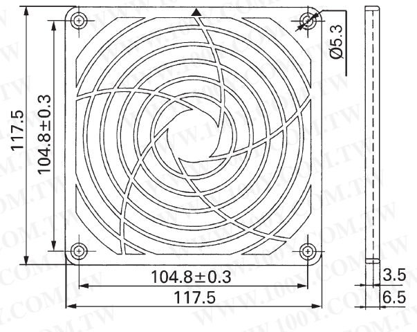
PG-12 (For UF12A, 12B Series) *Plastic
