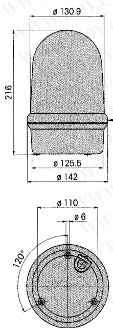
Rotating Mirror Beacon
