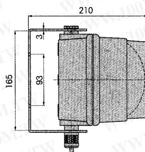
Signal Beacon
