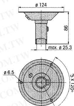
975 883 02 Flange for tube mounting
