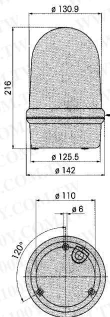
Revolving Signal Beacon
