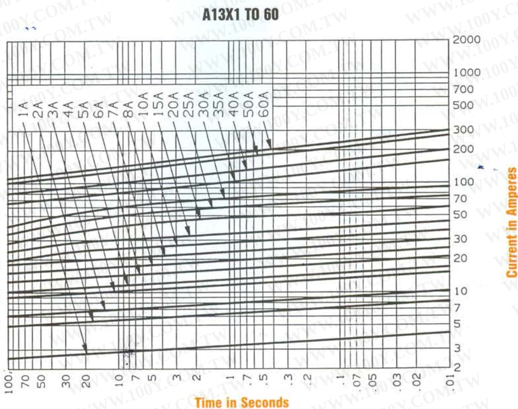
Melting Time - Current Data, 130V Fuses
