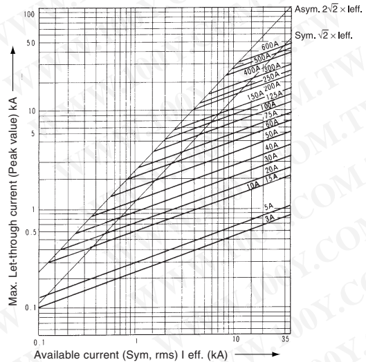
Current limiting characteristic
