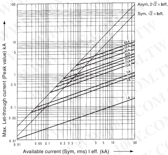
Current limiting characteristic
