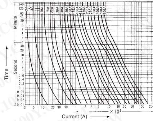
Permissible time-current characteristic
