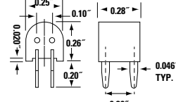
Circuit Board Mounting Detail
