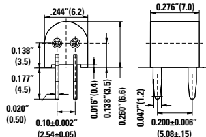
Circuit Board Mounting Detail
