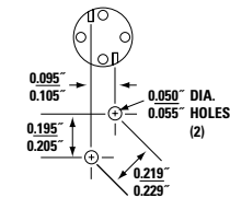
Circuit Board Mounting Detail
