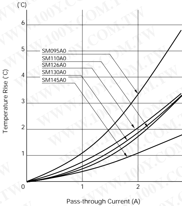
Temperature Rise
