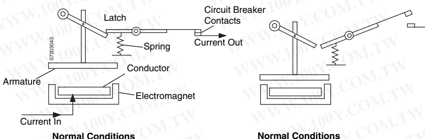
Figure 2: Magnetic Tripping
