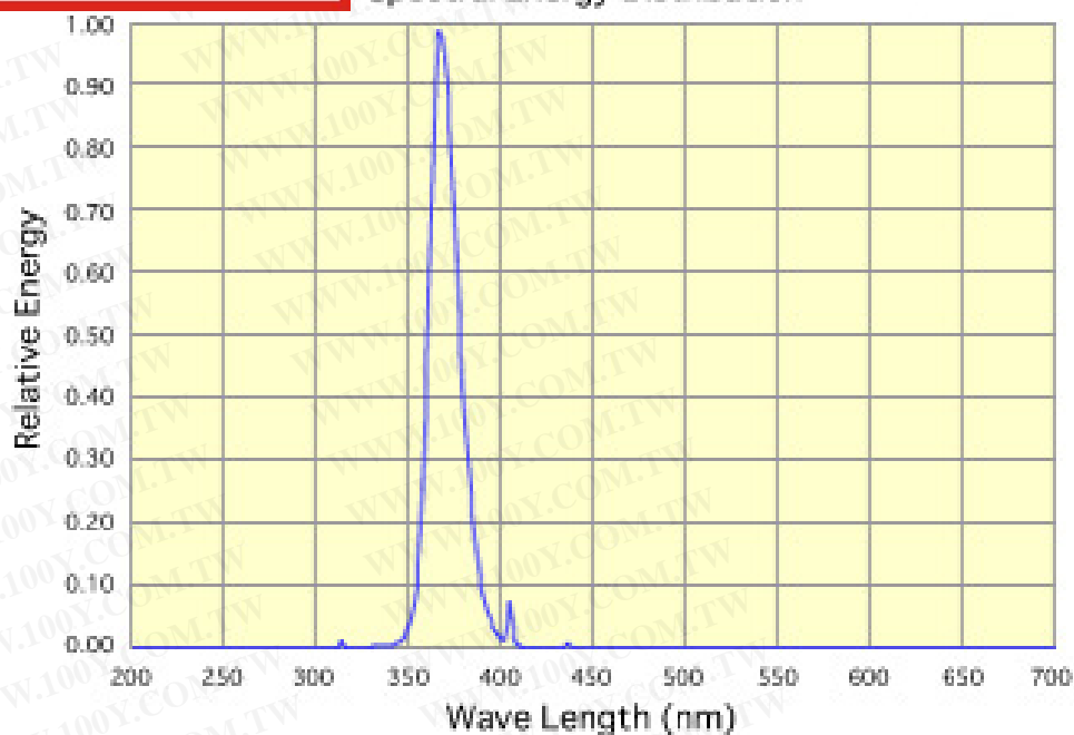
Spectral Energy Distribution
