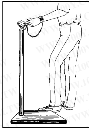
Figure 11. Testing of wrist strap grounding assemblies
