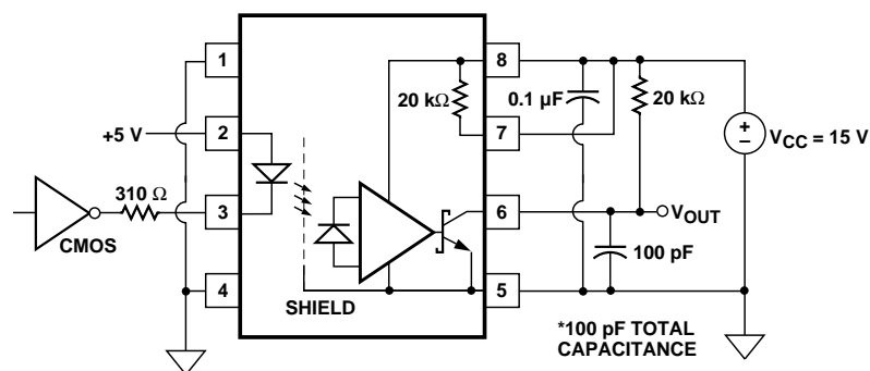
Figure 19. Recommended LED Drive Circuit.
