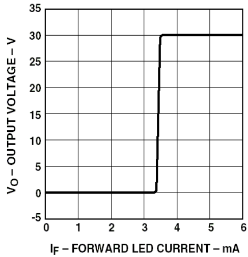
Figure 15. Transfer Characteristics.
