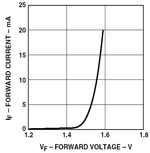
Figure 16. Input Current vs. Forward Voltage.
