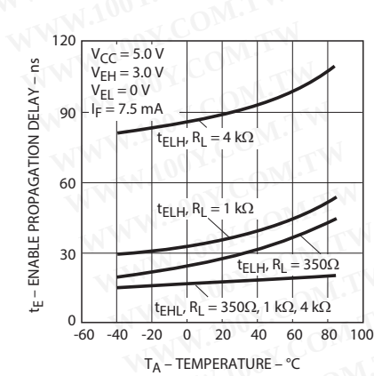
Figure 14: Typical Enable Propagation Delay vs. Temperature
