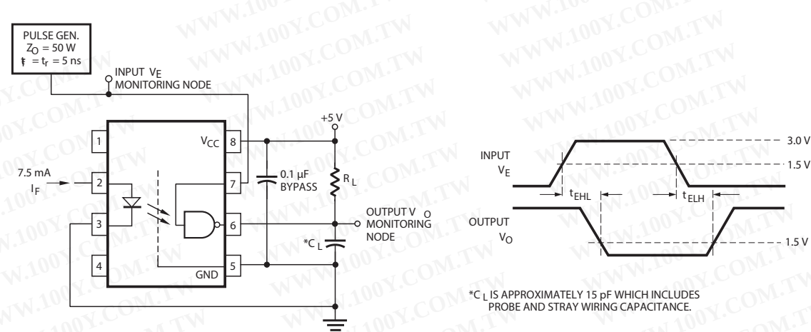
Figure 13: Test Circuit for t_{EHL} and t_{ELH}
