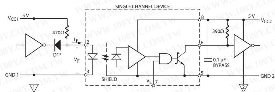
Figure 17: Recommended TTL/LSTTL to TTL/LSTTL Interface Circuit
