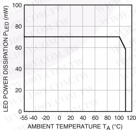
Fig. 12 LED Power Dissipation vs. Ambient Temperature (FOD817)
