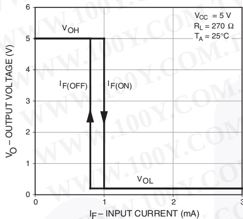
Figure 3. Transfer Characteristics
