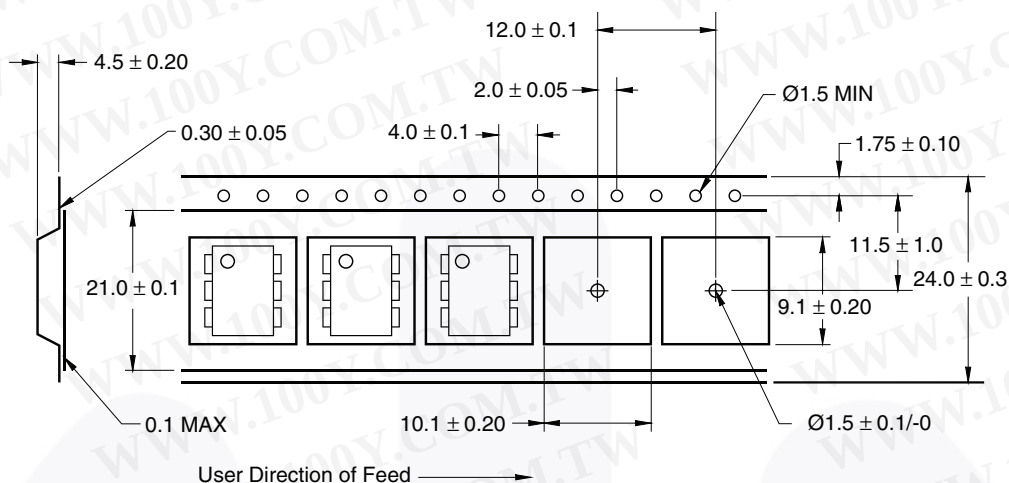
Figure 14. Tape Dimensions
