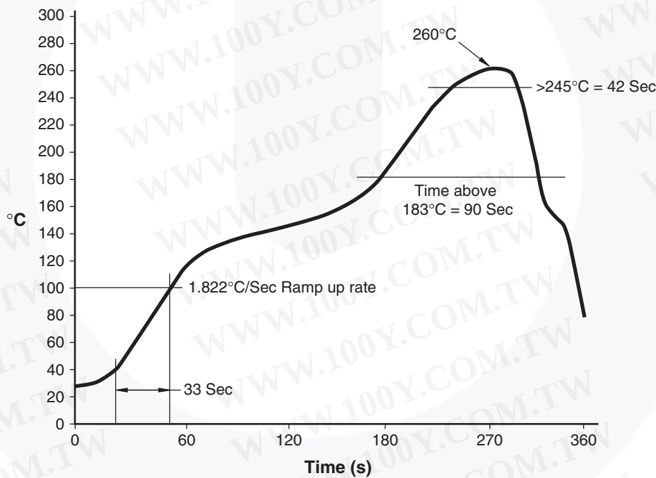
Figure 10. Reflow Profile
