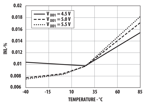
Figure 6. INL (%) vs. Temperature
