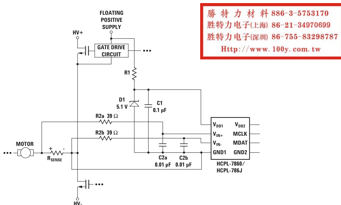
Figure 19. Schematic for Three Conductor Shunt Connection.
