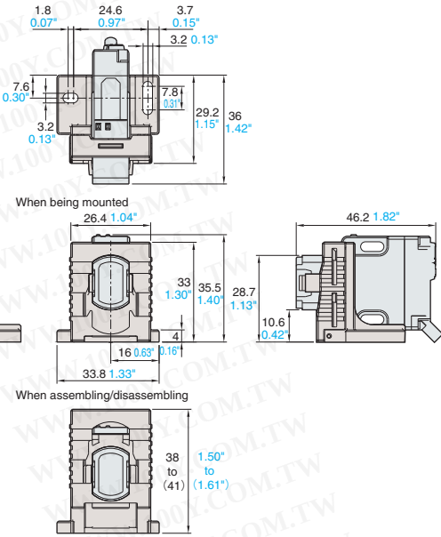
PZ-B82+PZ-G41B
