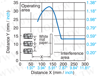
PZ-G42
