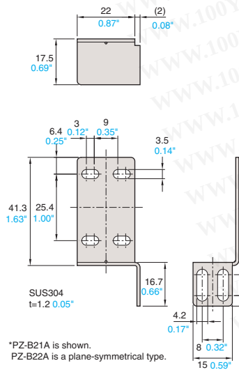
PZ-B21A/B22A
