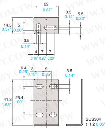
PZ-B01A
