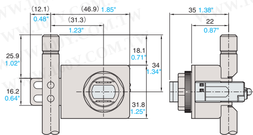
PZ-S□A+PZ-B25+PZ-G41B
