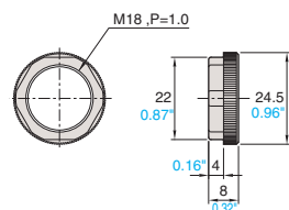
OP-84225
