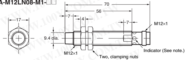
E2A-M12LN08-M1-□□
