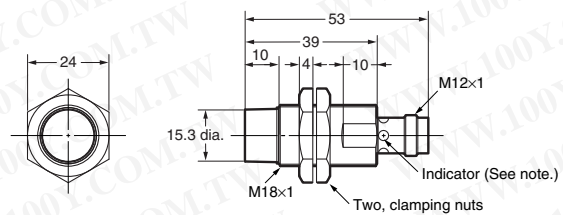
E2A-M18KN16-M1-□□
