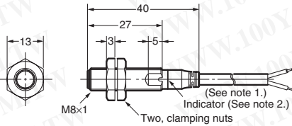
E2A-S08KS02-WP-□□
