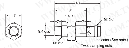
E2A-M12KN08-M1-□□
