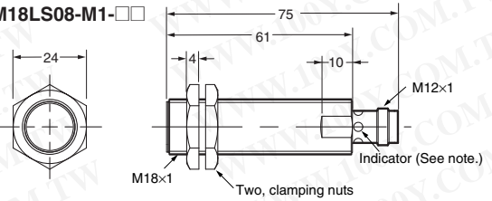
E2A-M18LS08-M1-□□
