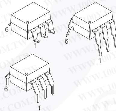
Figure 2. Package Outlines
