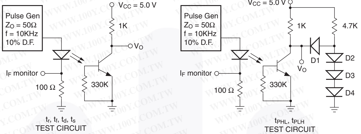
Figure 15. Switching Time Test Circuits
