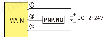
P Type
