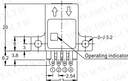
PNP Type
