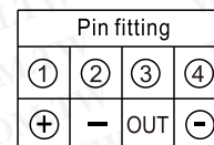
P Type
