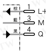
M8, 3-pin
