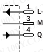
3-pin, M8
