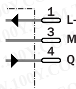
3-pin, M8
