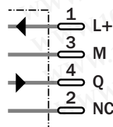
4-pin, M8
