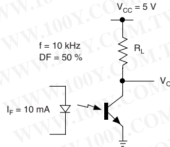
Fig. 14 - Switching Schematic
