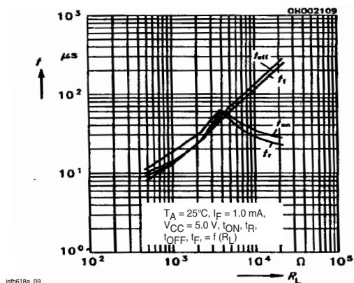
Figure 11. Switching times (typ.)
