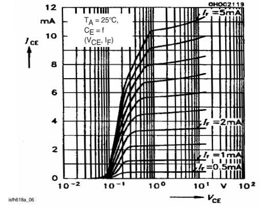
Figure 8. Output Characteristics
