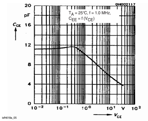
Figure 7. Transistor Capacitance
