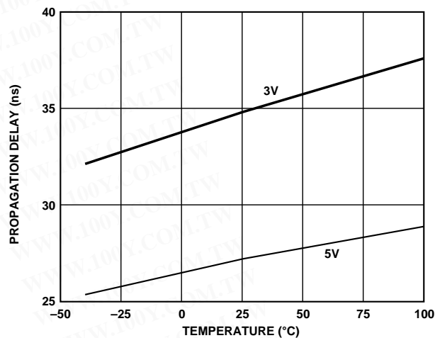
Figure 16. Propagation Delay vs. Temperature, C Grade
