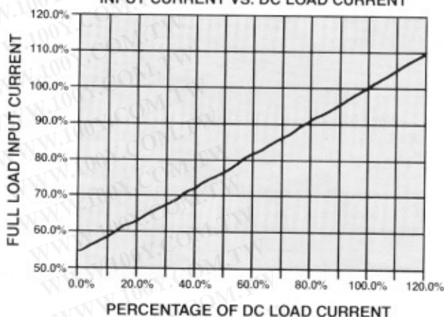
INPUT CURRENT VS. DC LOAD CURRENT
