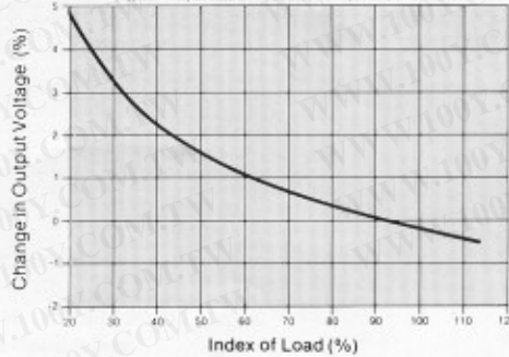
CHANGE IN OUTPUT VOLTAGE VS. LOAD
