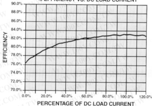
% EFFICIENCY VS. DC LOAD CURRENT
