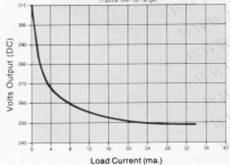
OUTPUT VOLTAGE VS. LOAD
