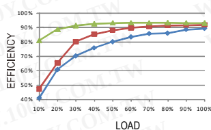
RSD-150C-12
