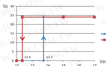
RSD-150B-24
