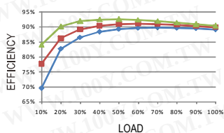
RSD-150D-5
