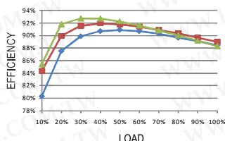
RSD-150C-5
