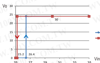
RSD-150C-24
