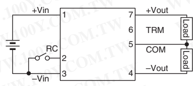
Terminal connections
