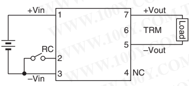
Connection diagram
