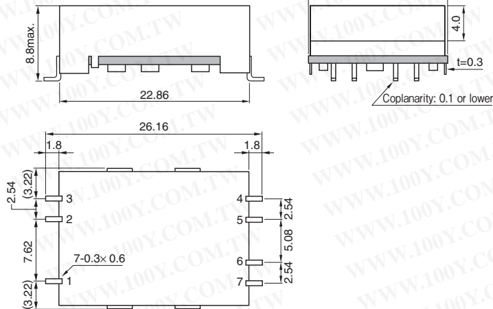
Shape/Dimensions
