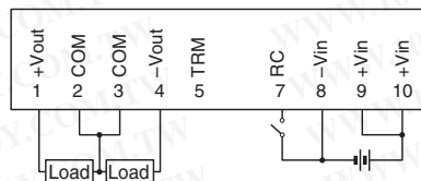
Terminal connections
