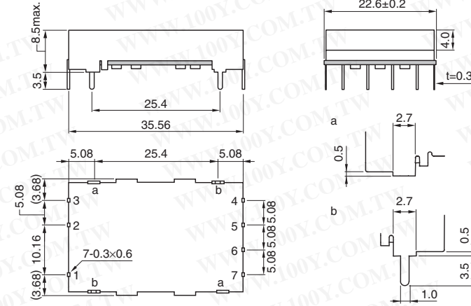
Shape/Dimensions
