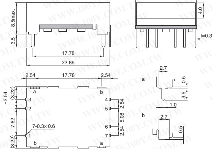
Shape/Dimensions
