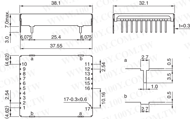
Shape/Dimensions
