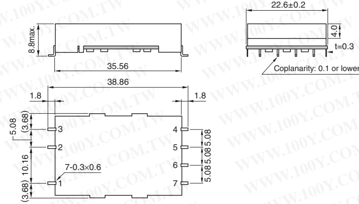
Shape/Dimensions
