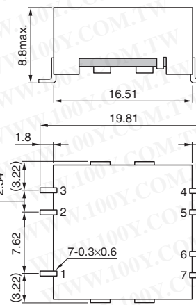
Shape/Dimensions
