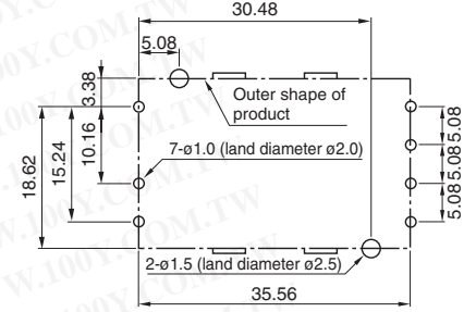
Recommended measurements for mounting board
