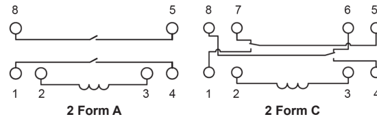
Schematic View
