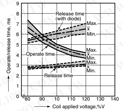
3. Operate/Release time (at 20°C 68°F)
