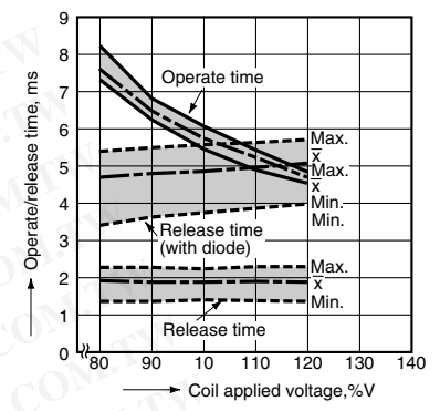
6. Operate/Release time (at 20°C 68°F)
