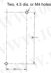
Mounting Holes
