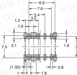
Mounting Dimensions (Top View) Tolerance: \pm 0.1 mm
