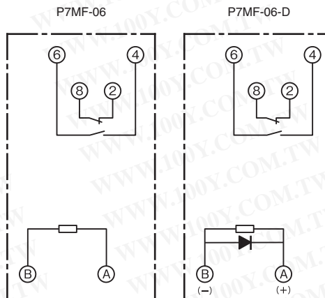
Terminal Arrangement/Internal Connections (TOP View)
