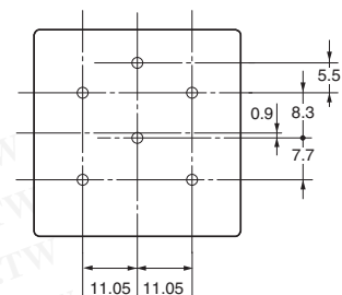
PCB Mounting Holes (Bottom View)
