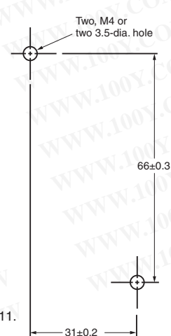
Mounting Holes (TOP View)
